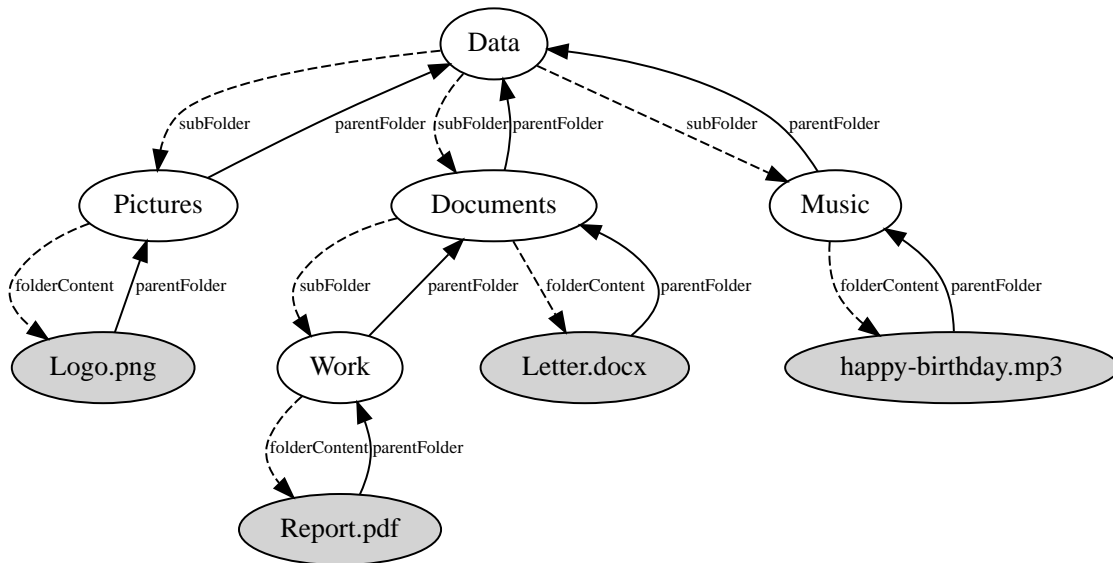
Figure 1. A simple file system graph with 9 items and 16 references.
