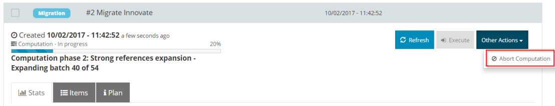
Figure 46. Abort an execution
